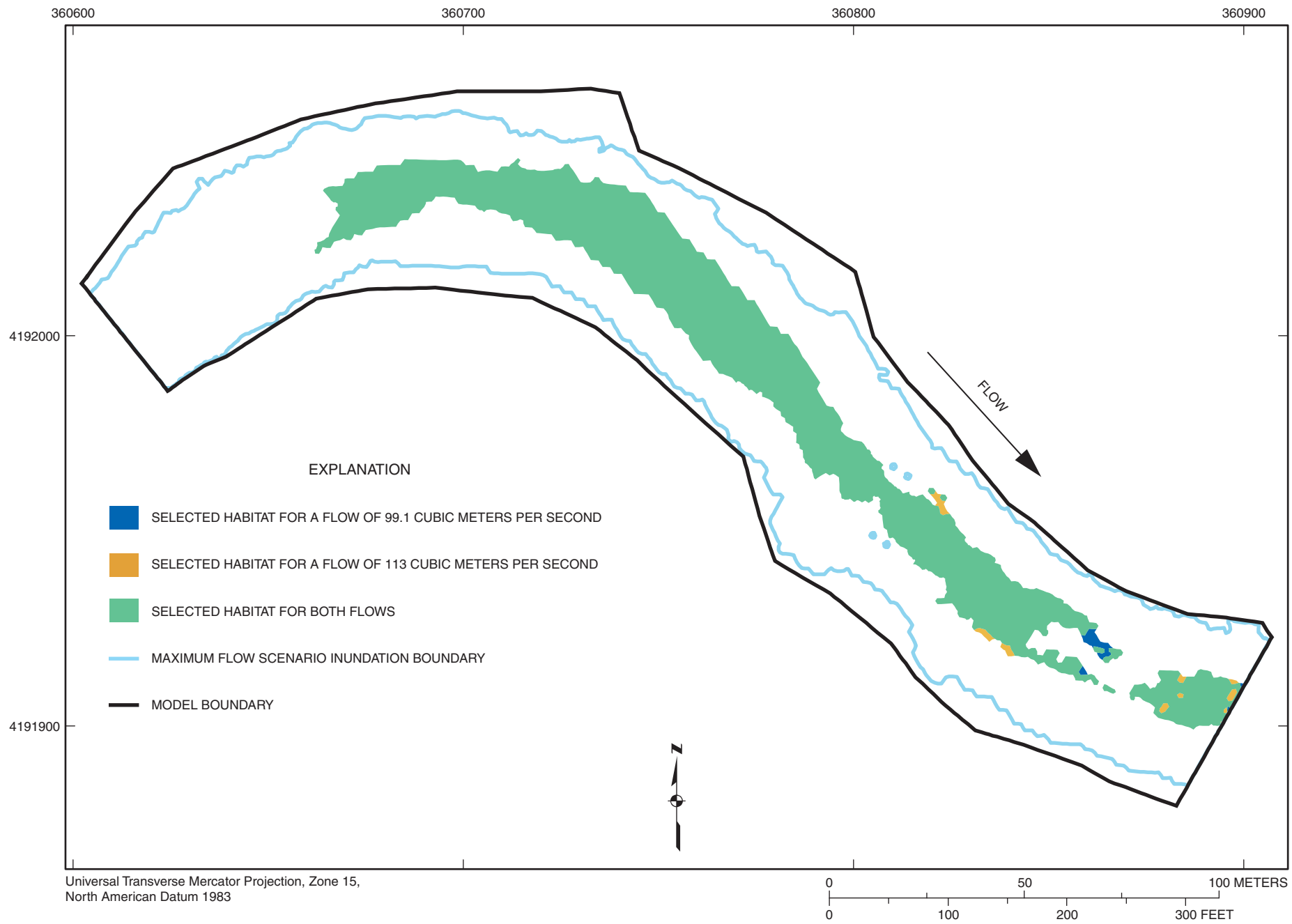
Figure 1-26. Selected habitat area distribution for habitat category 7 (paddlefish) at flows of 99.1 and 113 cubic meters per second at Marmaton River site M1.
